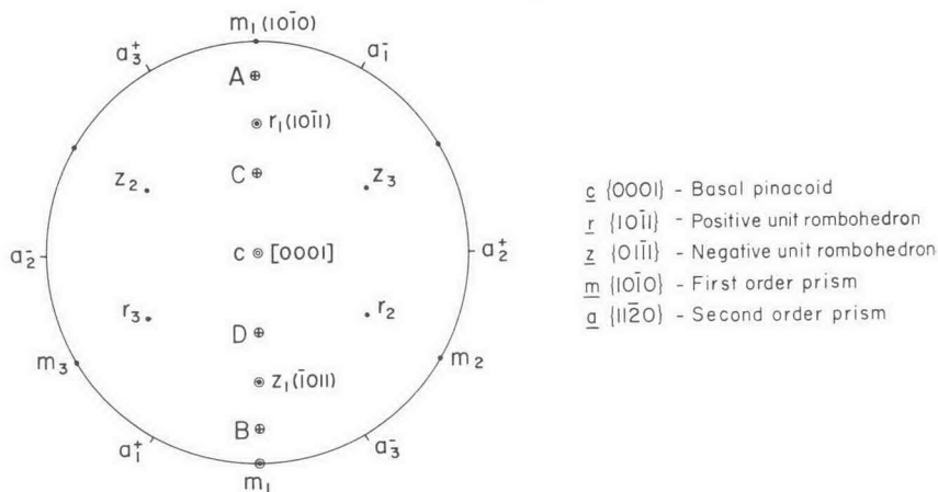
Fig. 3. Equal-area projection (lower hemisphere) showing the common crystal planes of quartz and the convention regarding polarity of the a -axes. Directions in which samples were cored are represented by circles.
