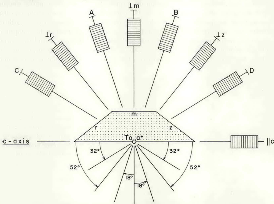
Fig. 4. Diagram representing the crystallographic orientations of the eight types of samples used in the experiments. The crystal is viewed towards the positive end of an a -axis.
